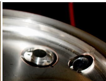
Completed assy showing copper braze & tacks
