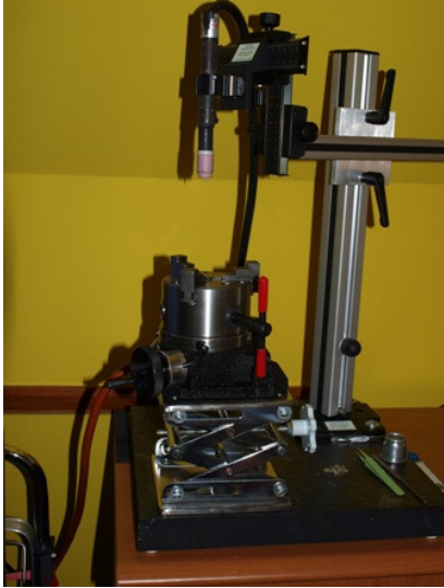
Full adjustable welding station for micro TIG welding
